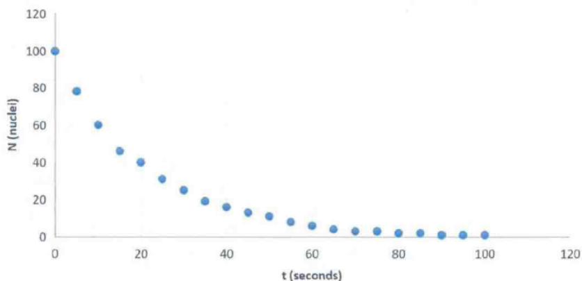
Number of present radioactive nuclei vs Time
