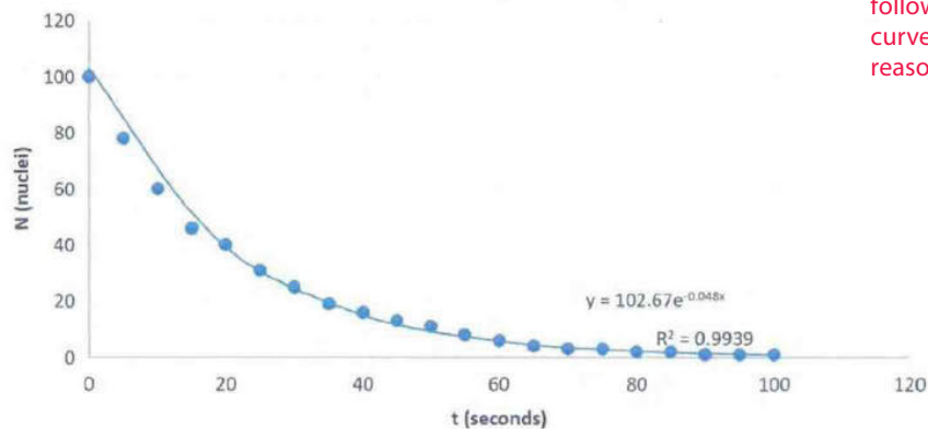
Figure 2. The relationship between the number of present radioactive nuclei and time
